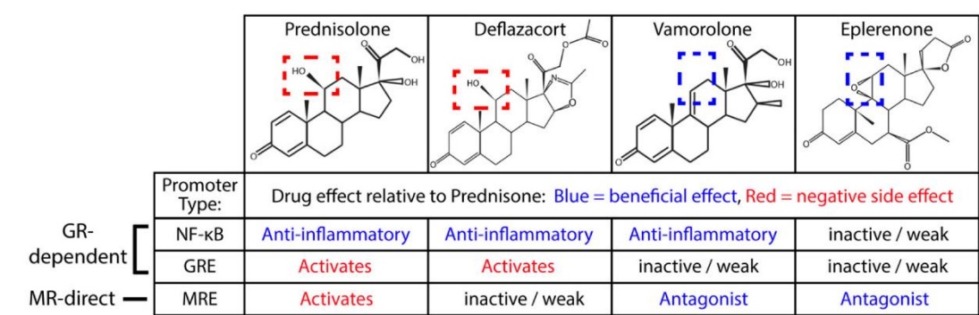
Figure 3: Molecular structure of vamorolone as compared to prednisone
